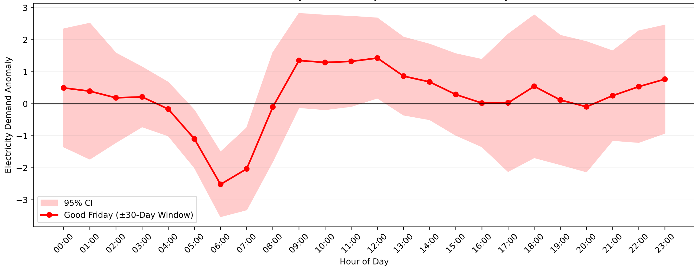
Avoca Demand Anomaly: Good Friday (2004-2017, \pm 30 -Day Window)
